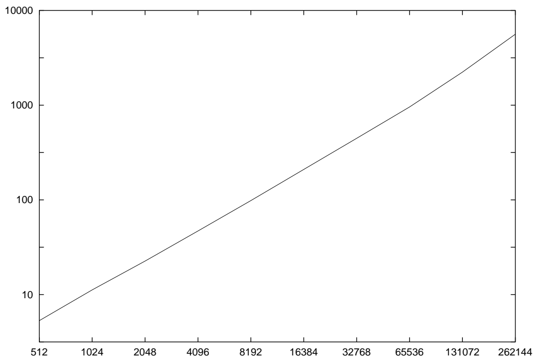
Fig 1. \log(\text{TIME}) versus \log(\text{SIZE}) .
